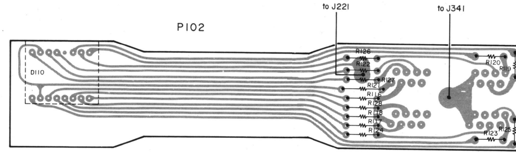
Figure 15 Seg Led Assembly-P102 Component Locations.
