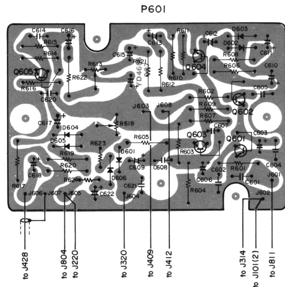
Figure 19 Mic/ALC Amp Assembly-P601 Component Locations.
