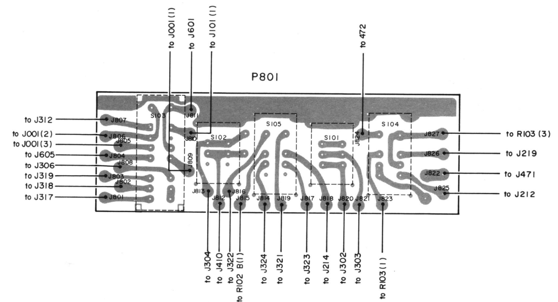
Figure 20 Switch Assembly-P801 Component Locations.
