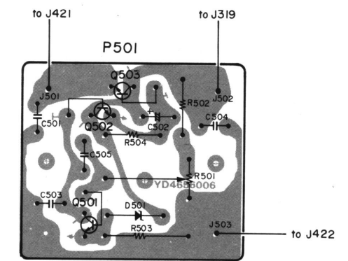
Figure 18 Regulator Assembly-P501 Component Locations.
