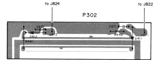
Figure 17 SWR Assembly-P302 Component Locations.
