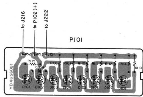
Figure 14 LID Assembly-P101 Component Locations.
