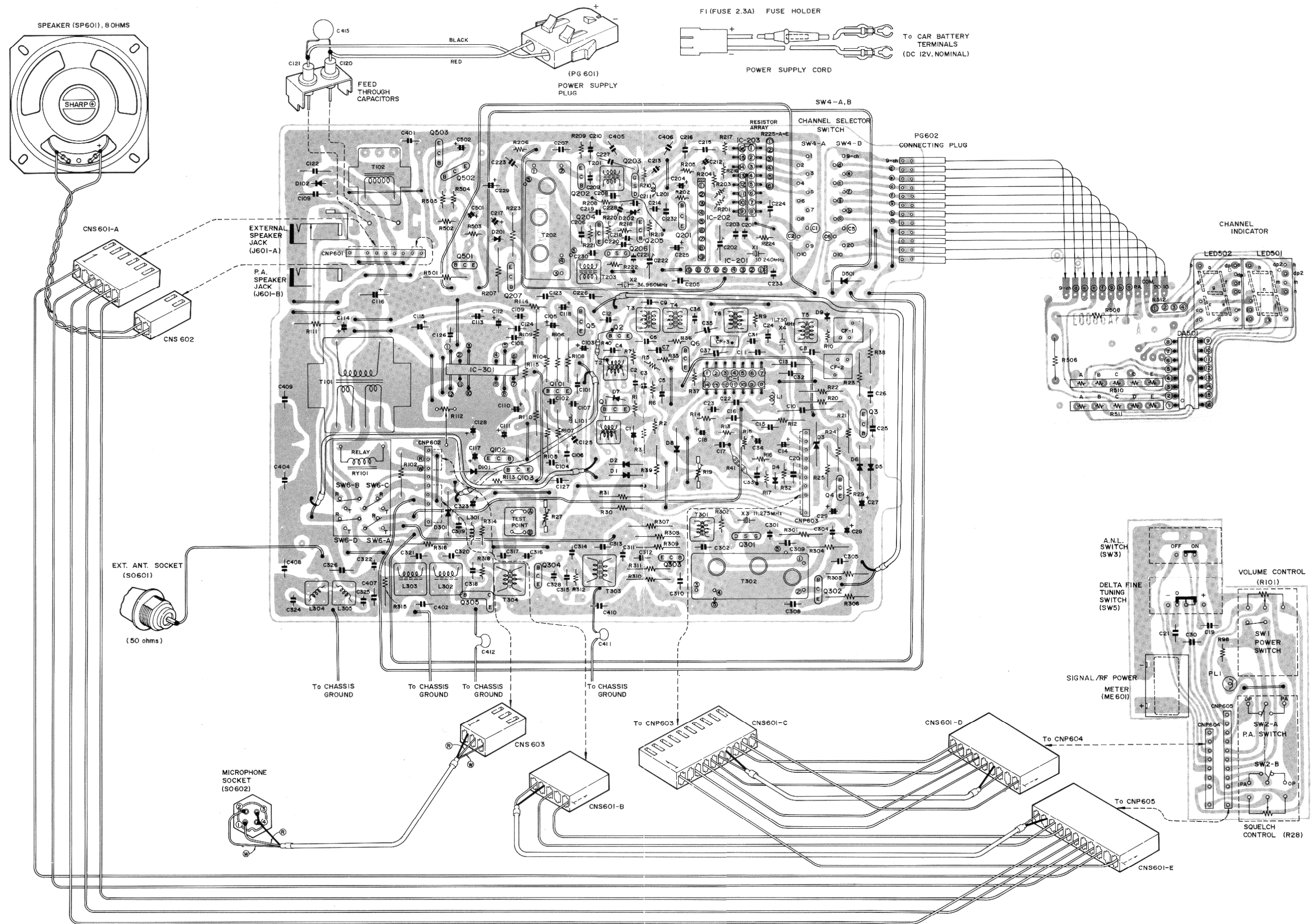
Figure 14 WIRING SIDE OF P.W. BOARD (NEW)
