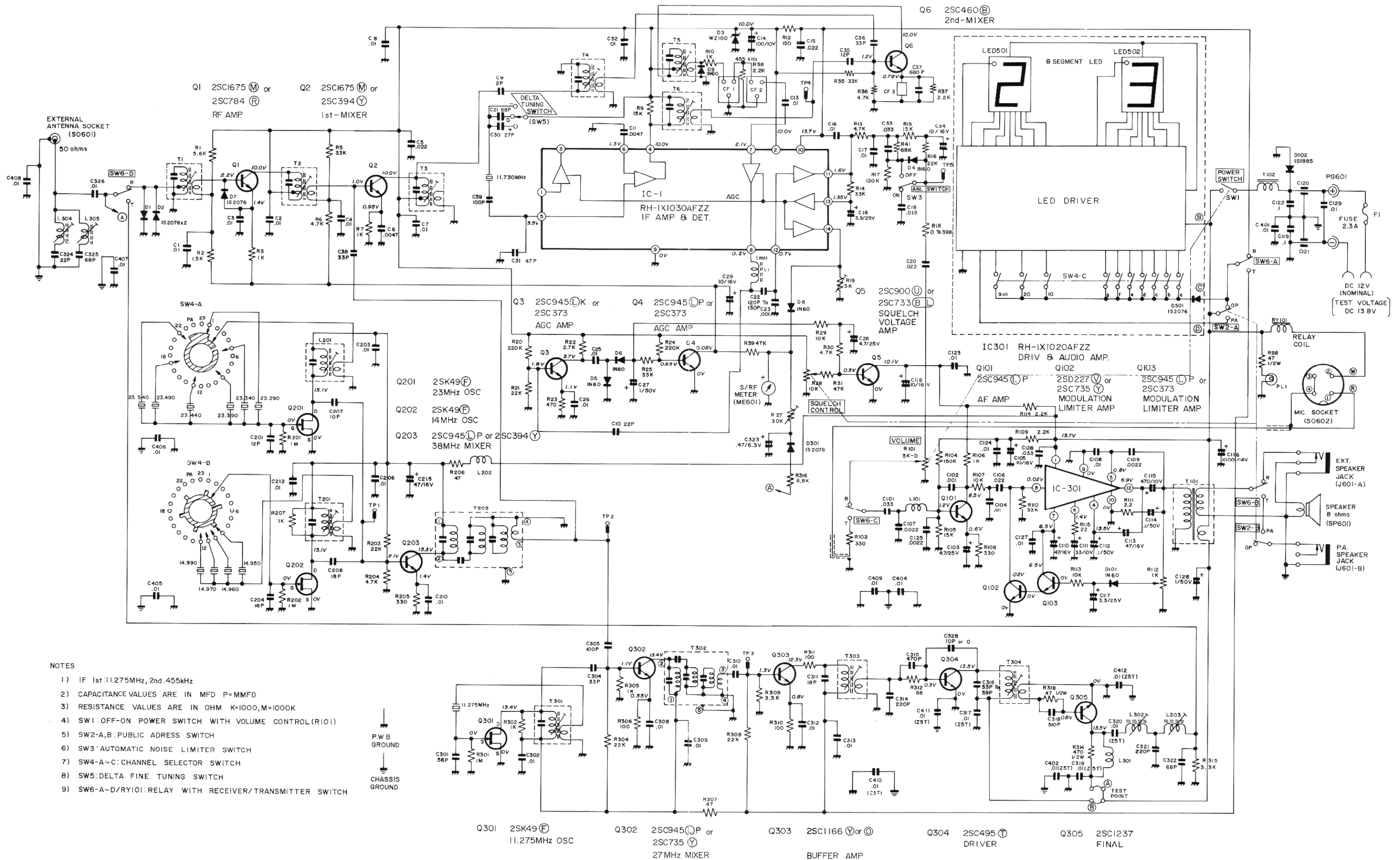
Figure 24 SCHEMATIC DIAGRAM (P.W.B. NO. F0552AF)
