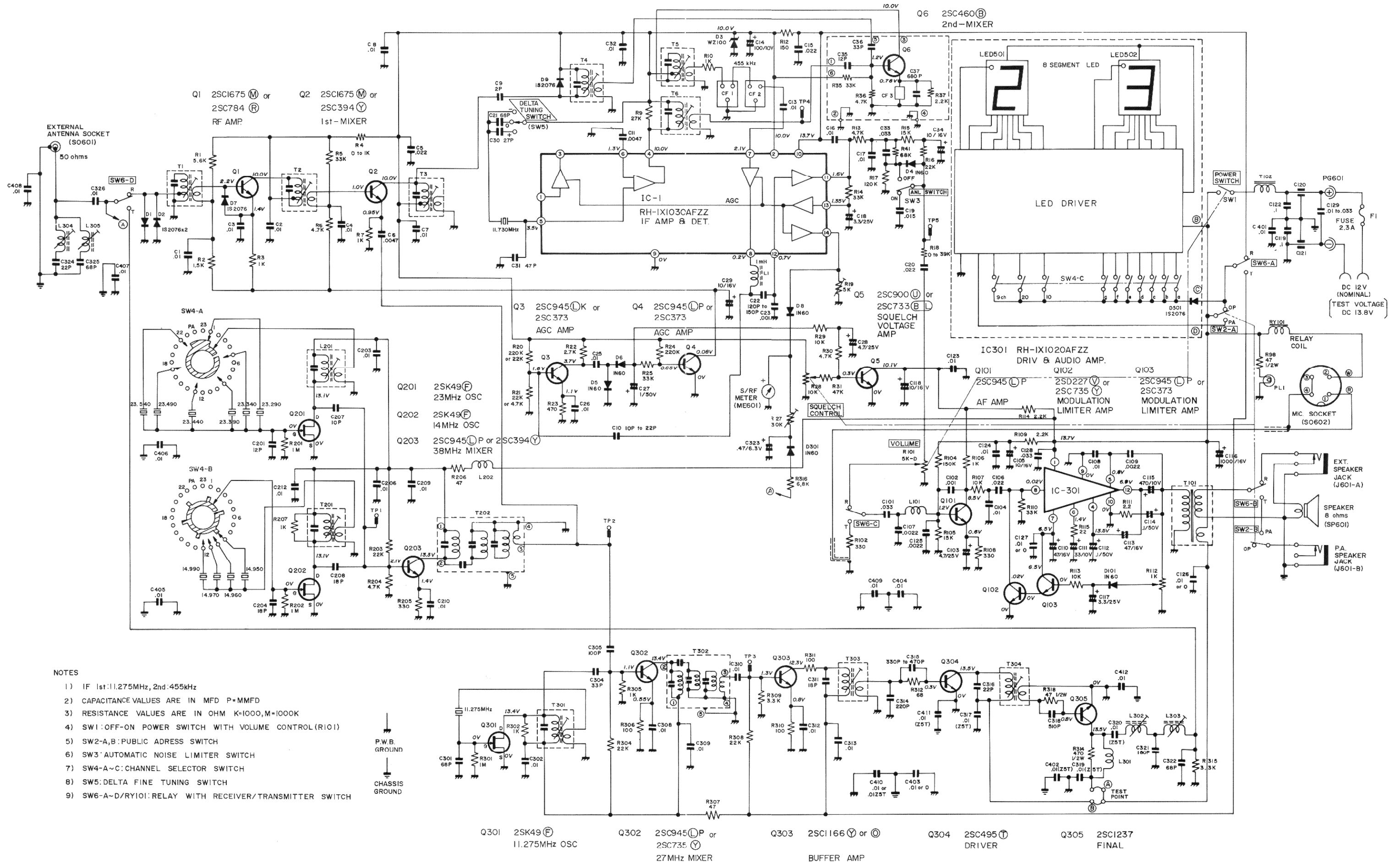
Figure 22 SCHEMATIC DIAGRAM (P.W.B. NO. F0485AF-5)
