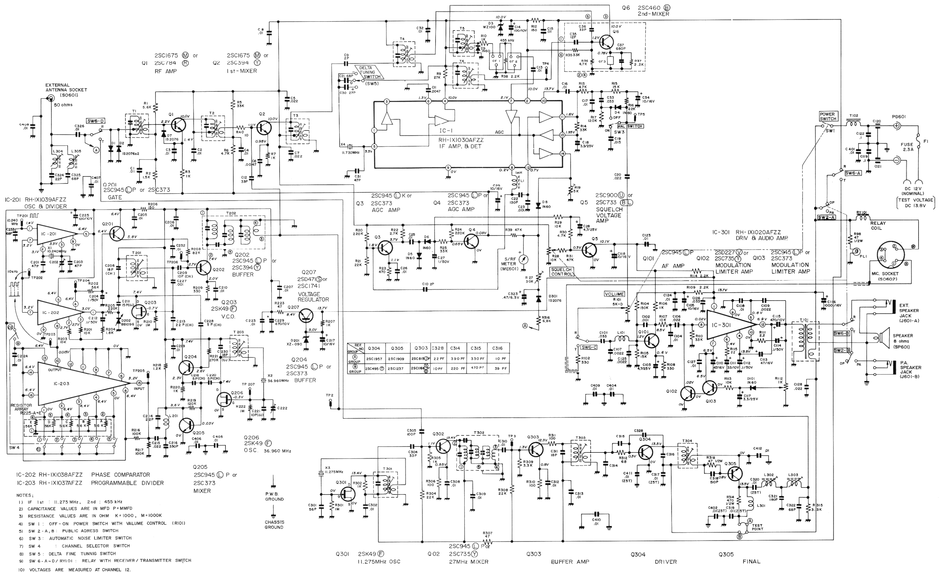
Figure 19 SCHEMATIC DIAGRAM
