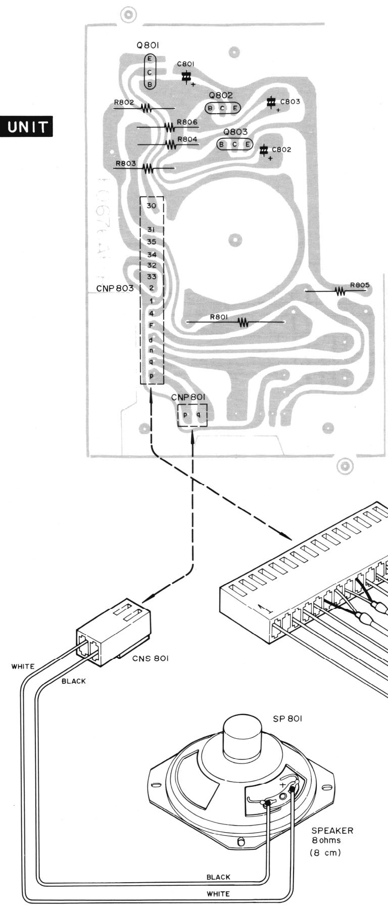
Figure 10 WIRING SIDE OF SPEAKER UNIT AND REMOTE MICROPHONE UNIT P.W. BOARDS
