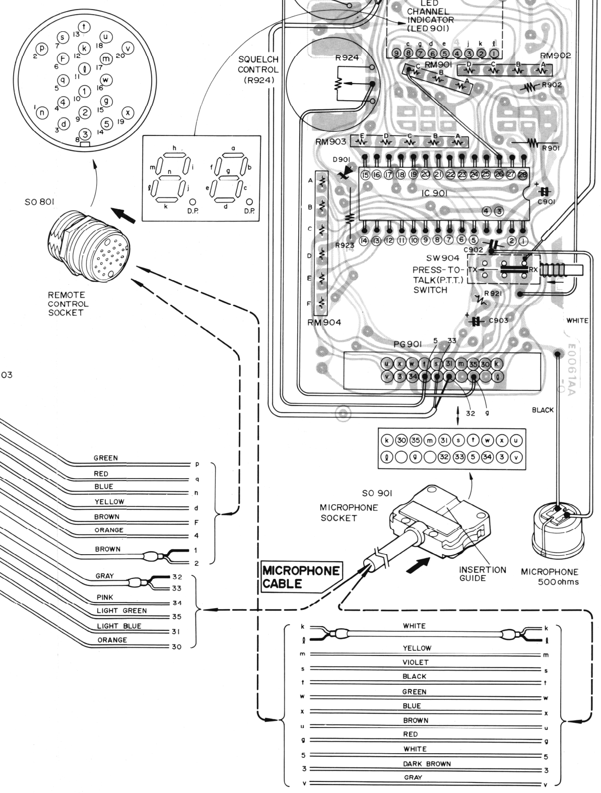
Figure 10 WIRING SIDE OF SPEAKER UNIT AND REMOTE MICROPHONE UNIT P.W. BOARDS
