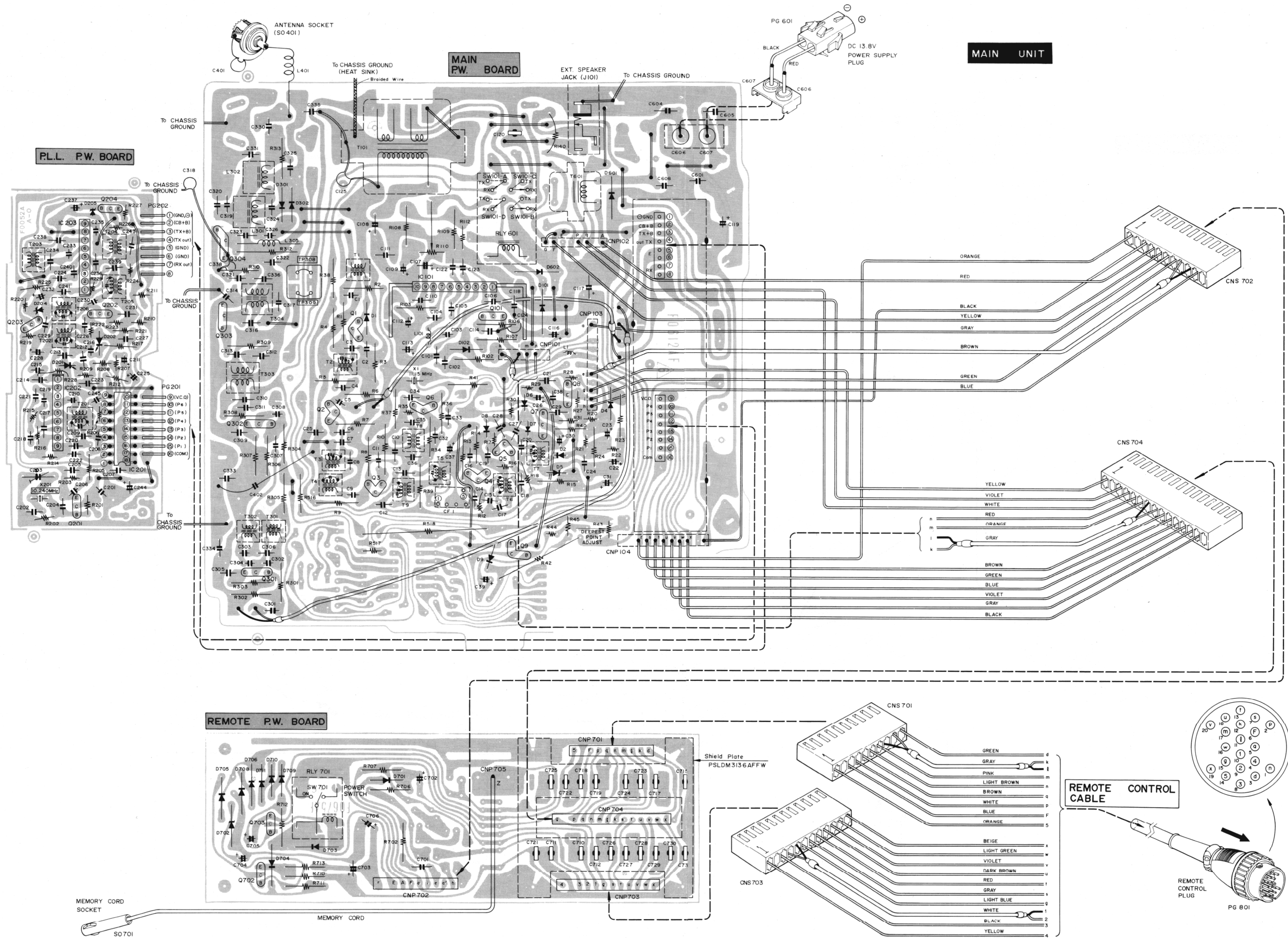
Figure 9 WIRING SIDE OF MAIN UNIT P.W. BOARDS
