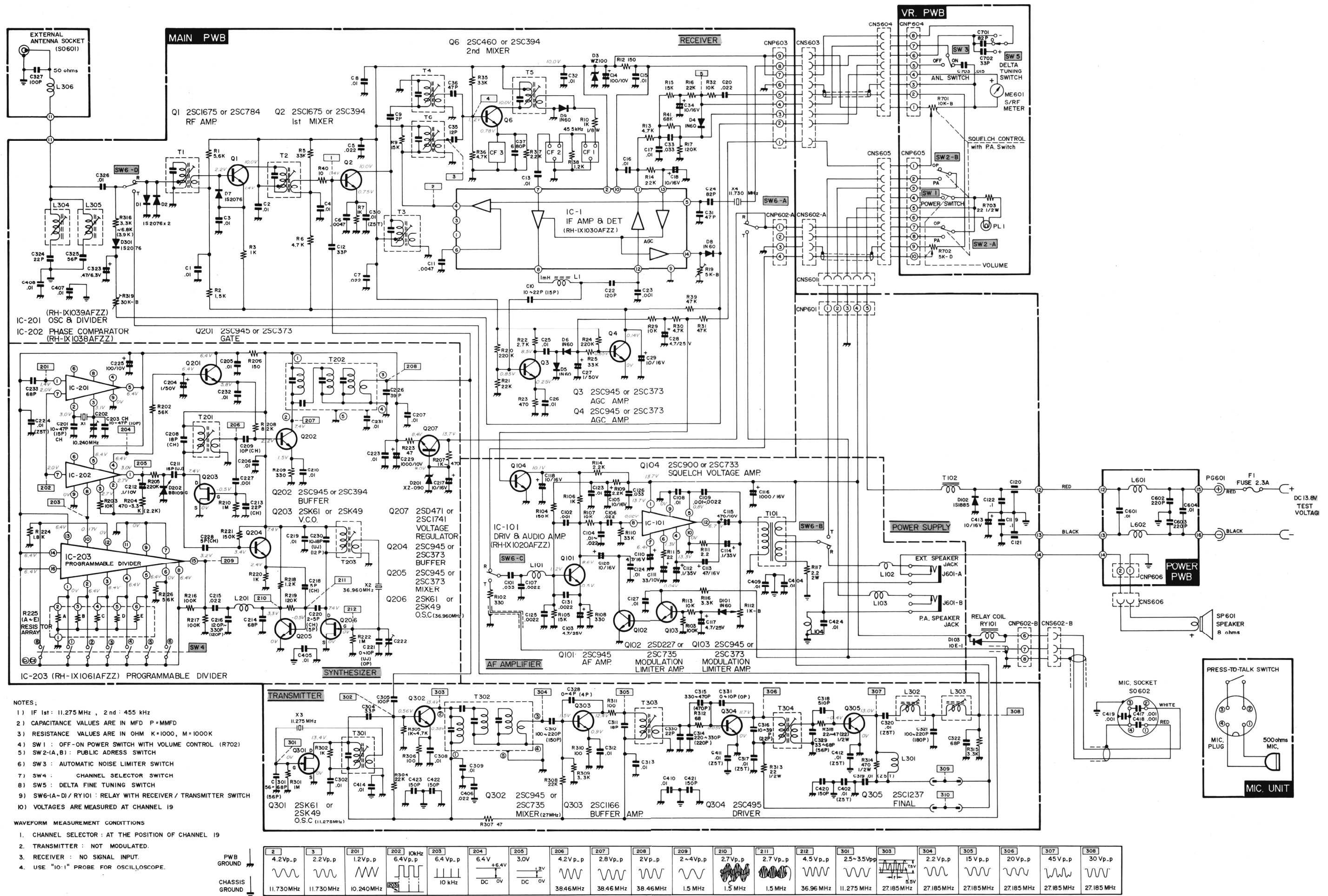
Figure 11 SCHEMATIC DIAGRAM
