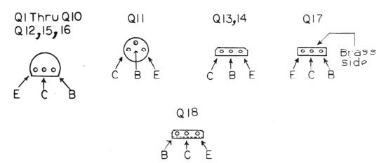
TRANSISTOR CASE DIAGRAMS (BOTTOM VIEW)
