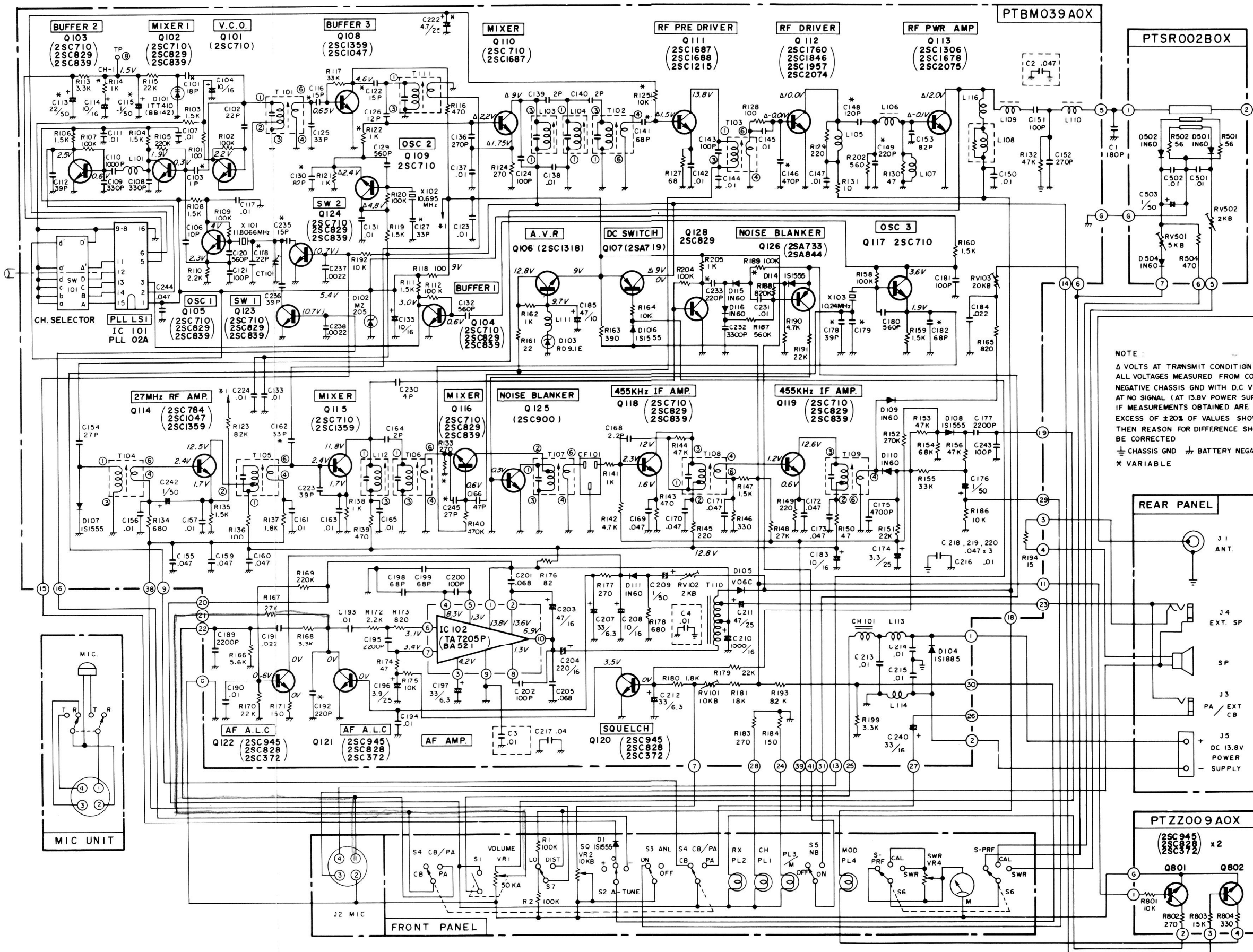
Figure 17 – Schematic Diagram of 14T301
