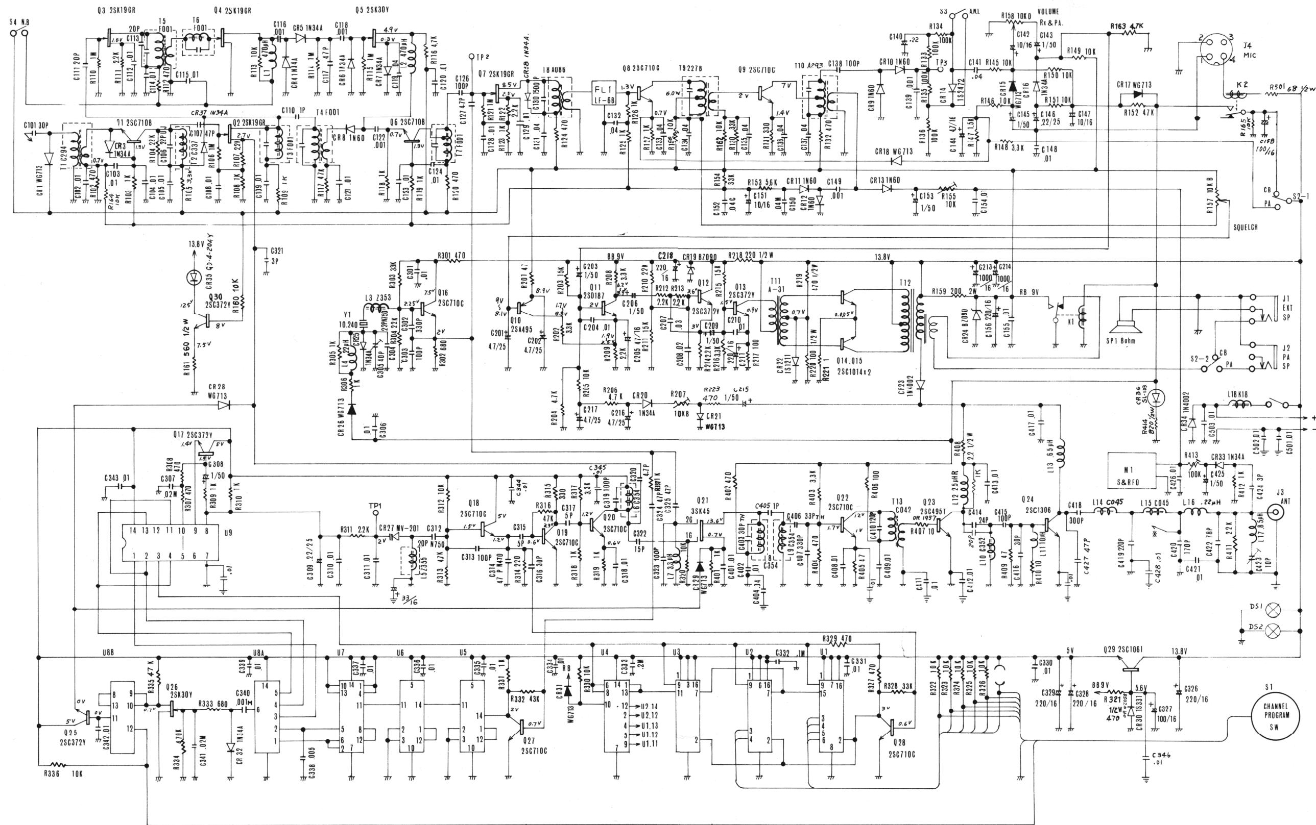
Figure 6-2 Schematic
