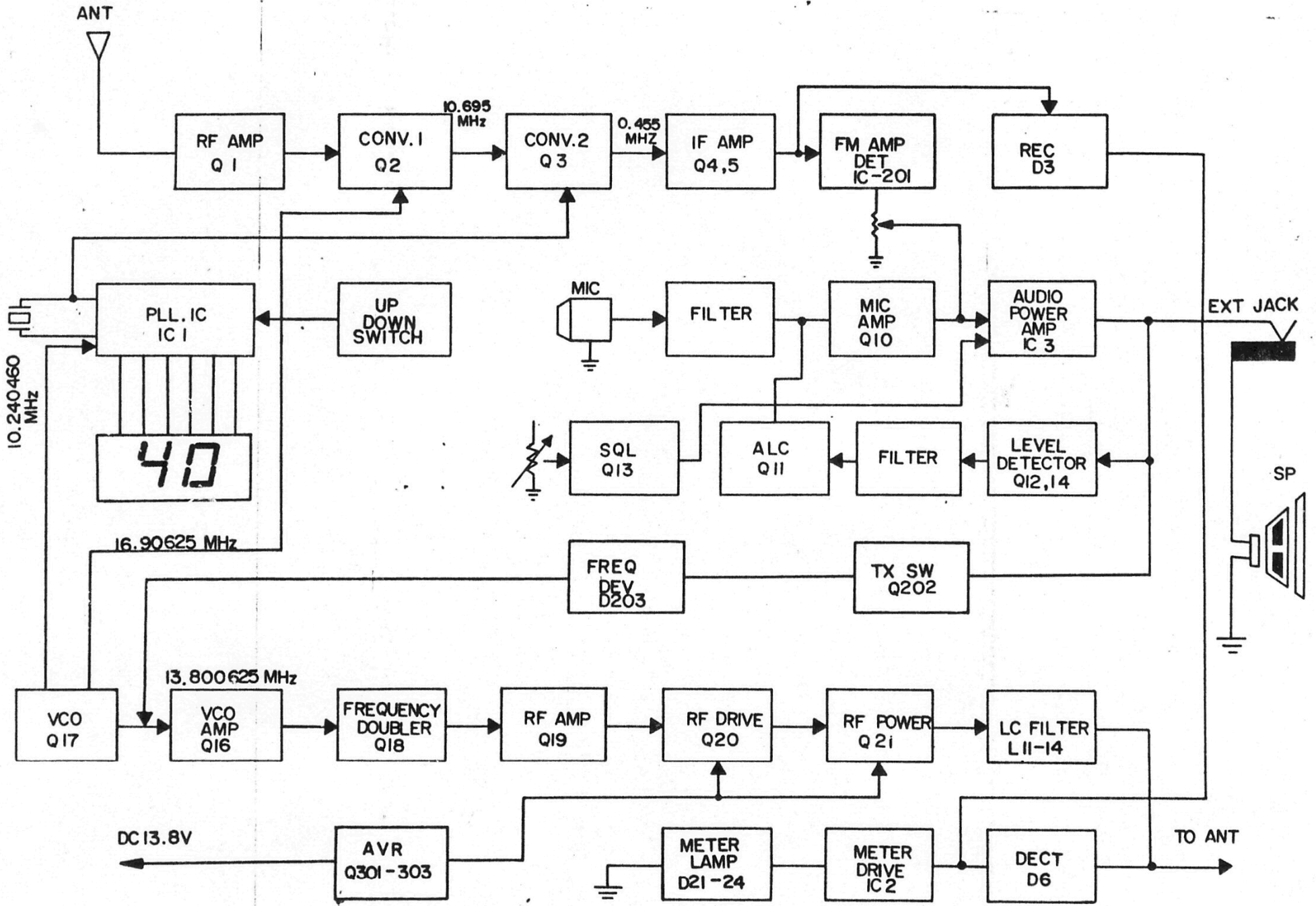
FUNCTIONAL BLOCK DIAGRAM
