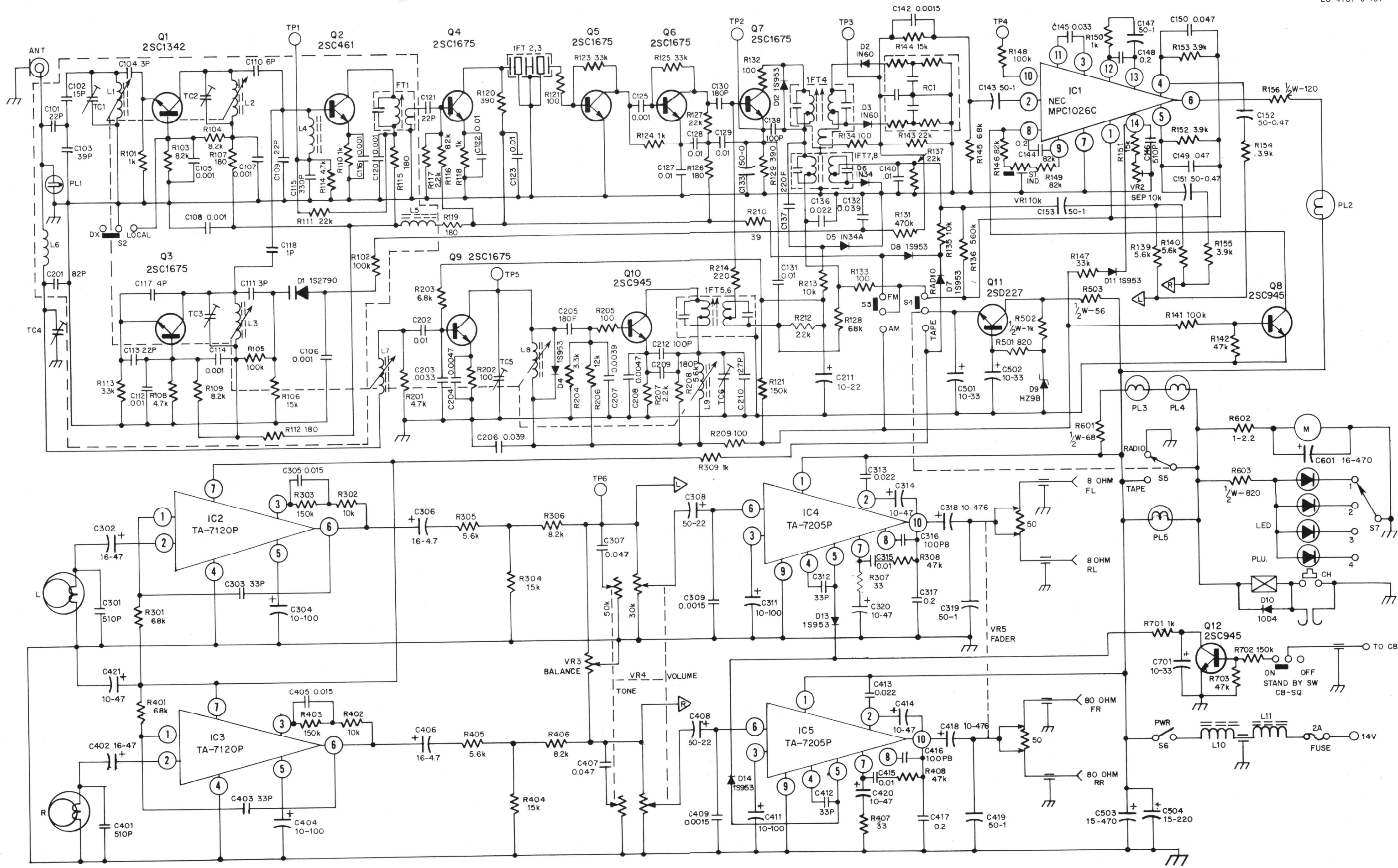
Figure 5-4. Schematic Diagram, Model 4701
