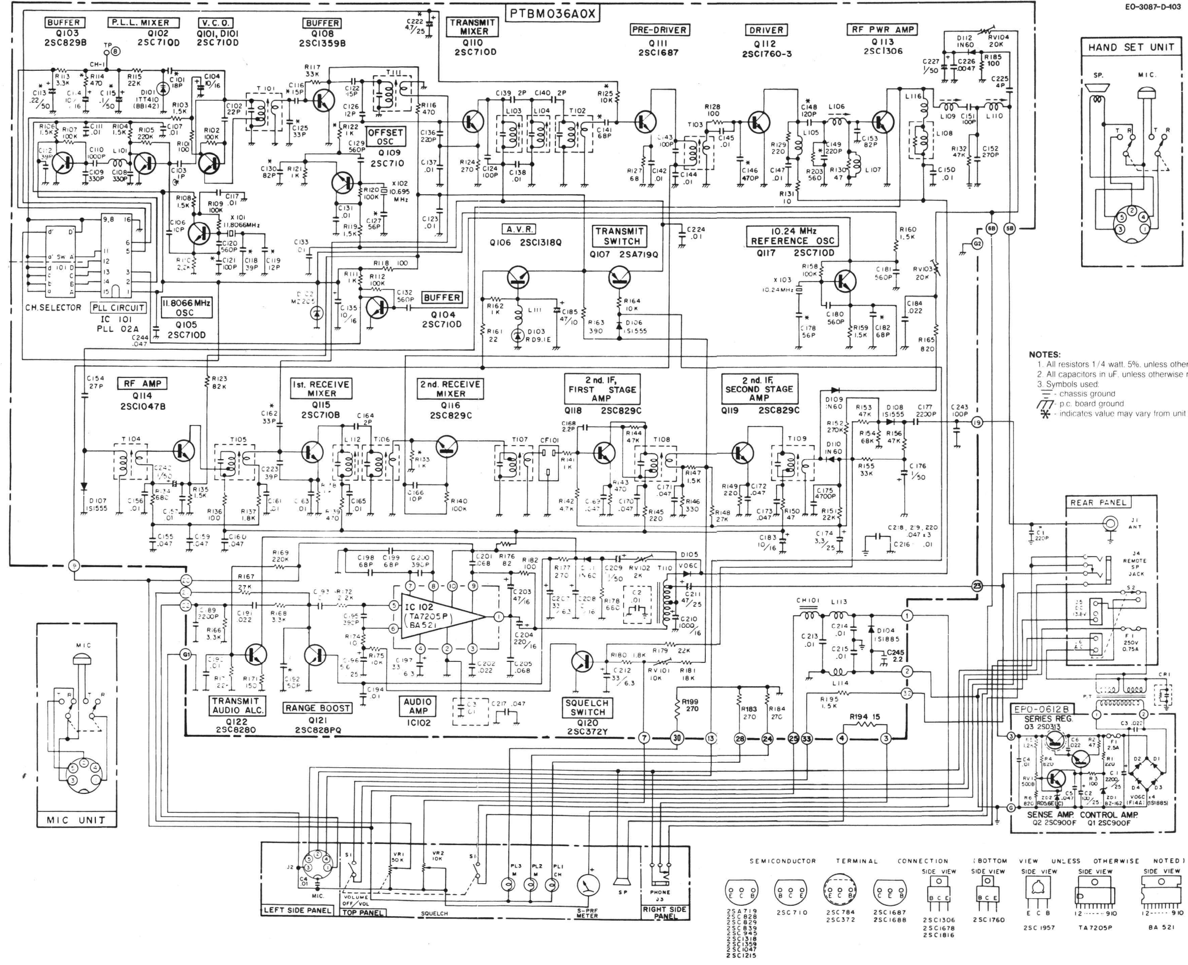
Figure 4-3. Schematic Diagram, Model 3087
