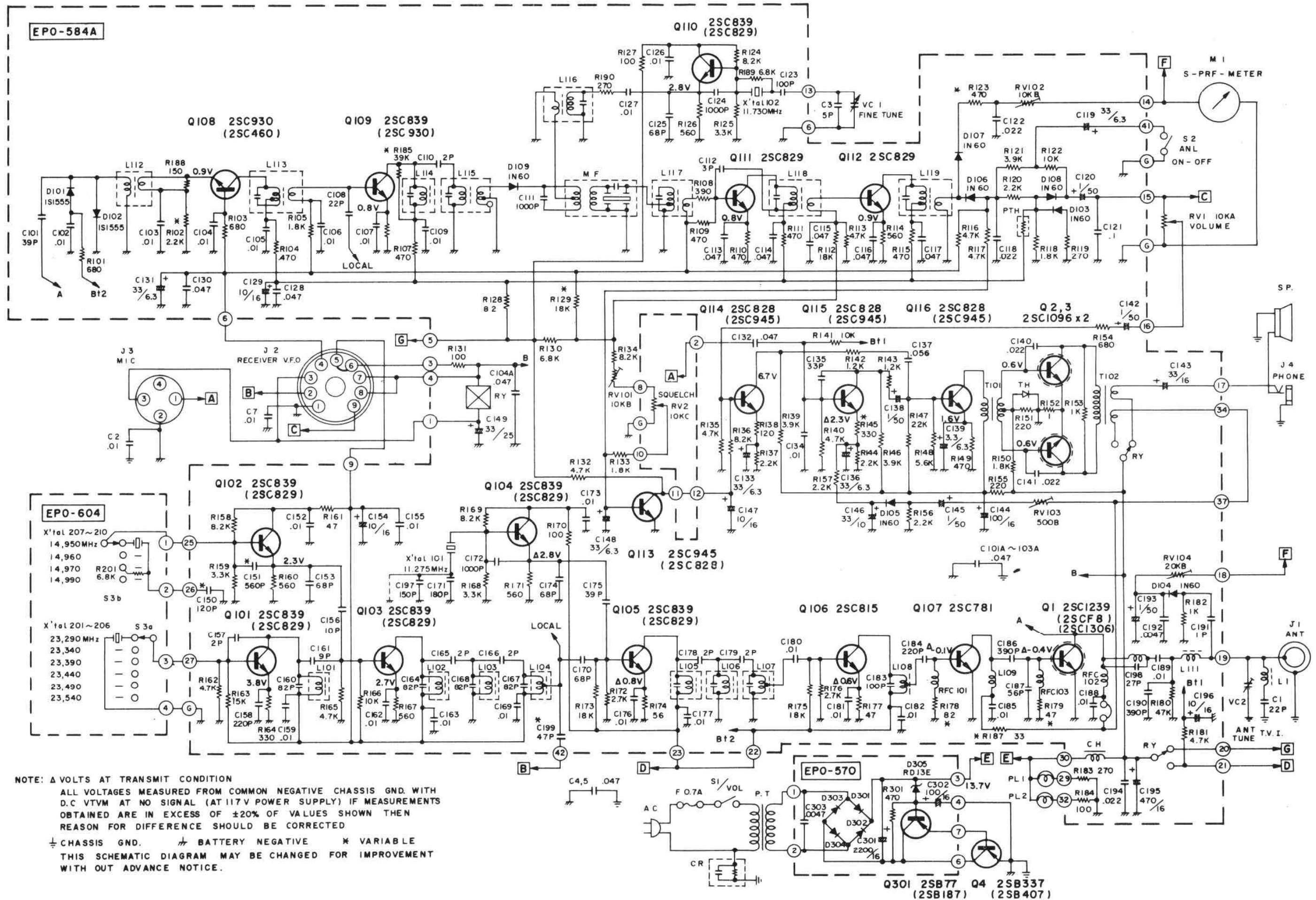
SCHEMATIC DIAGRAM HY-GAIN 673
