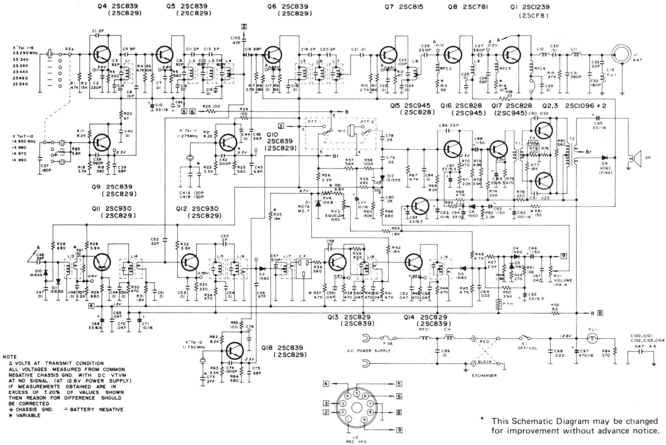
SCHEMATIC DIAGRAM OF MODEL 670
