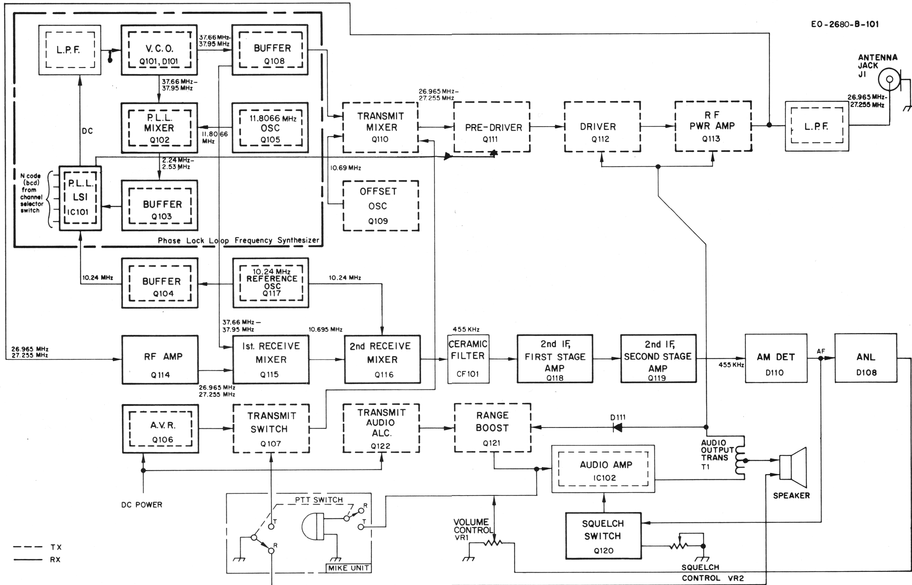
Figure 2-2. Block Diagram, Model 2680
