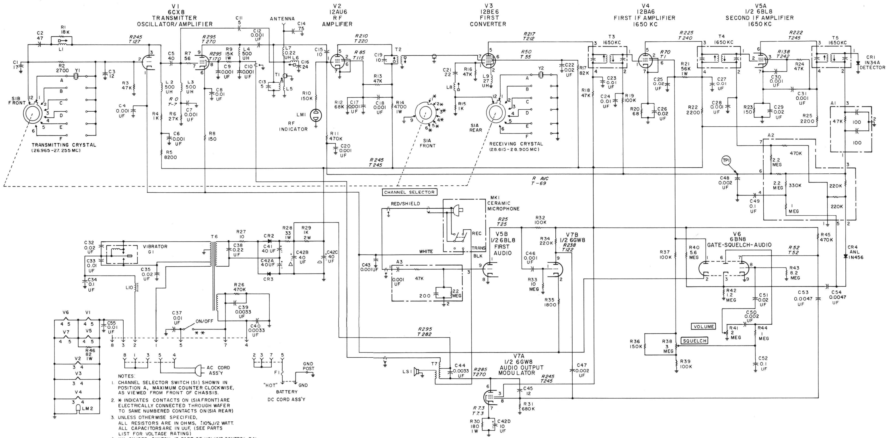
Model CB-17 Schematic Diagram
