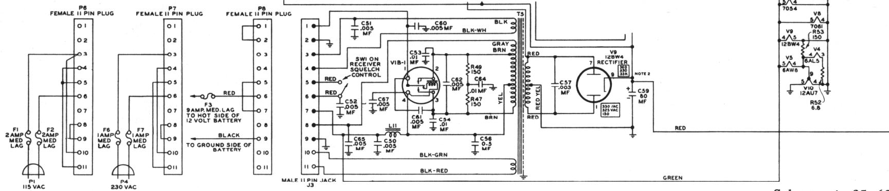
Schematic 25.638
