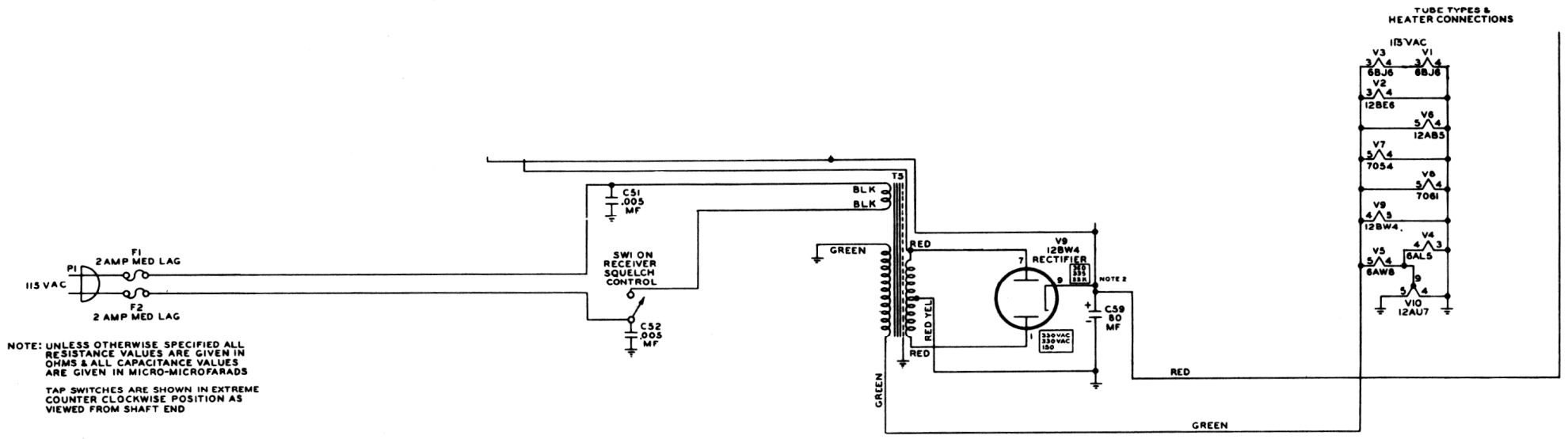
Schematic 25.526
