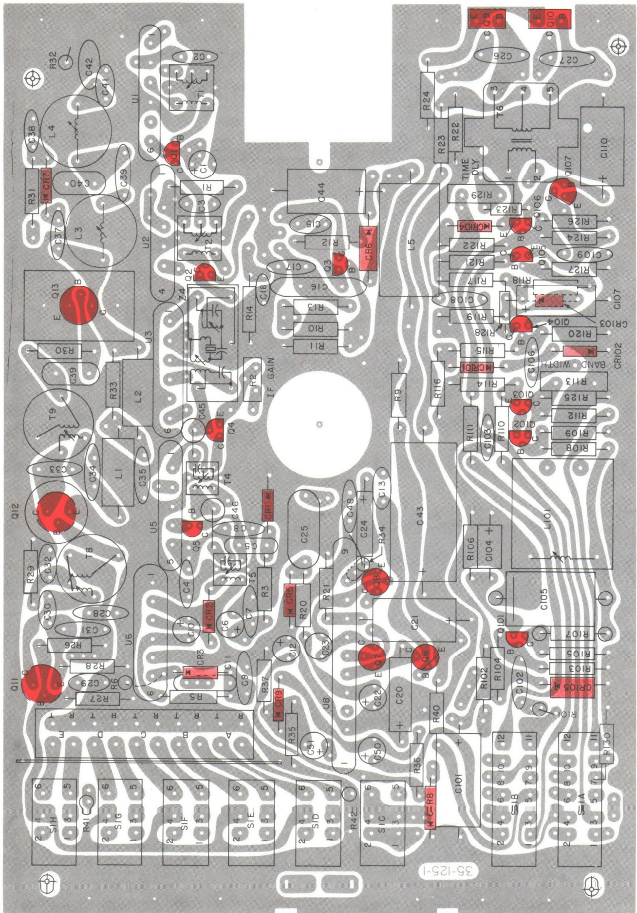
MESSENGER 120 PARTS LAYOUT (AS VIEWED FROM SOLDER SIDE OF PC BOARD)
