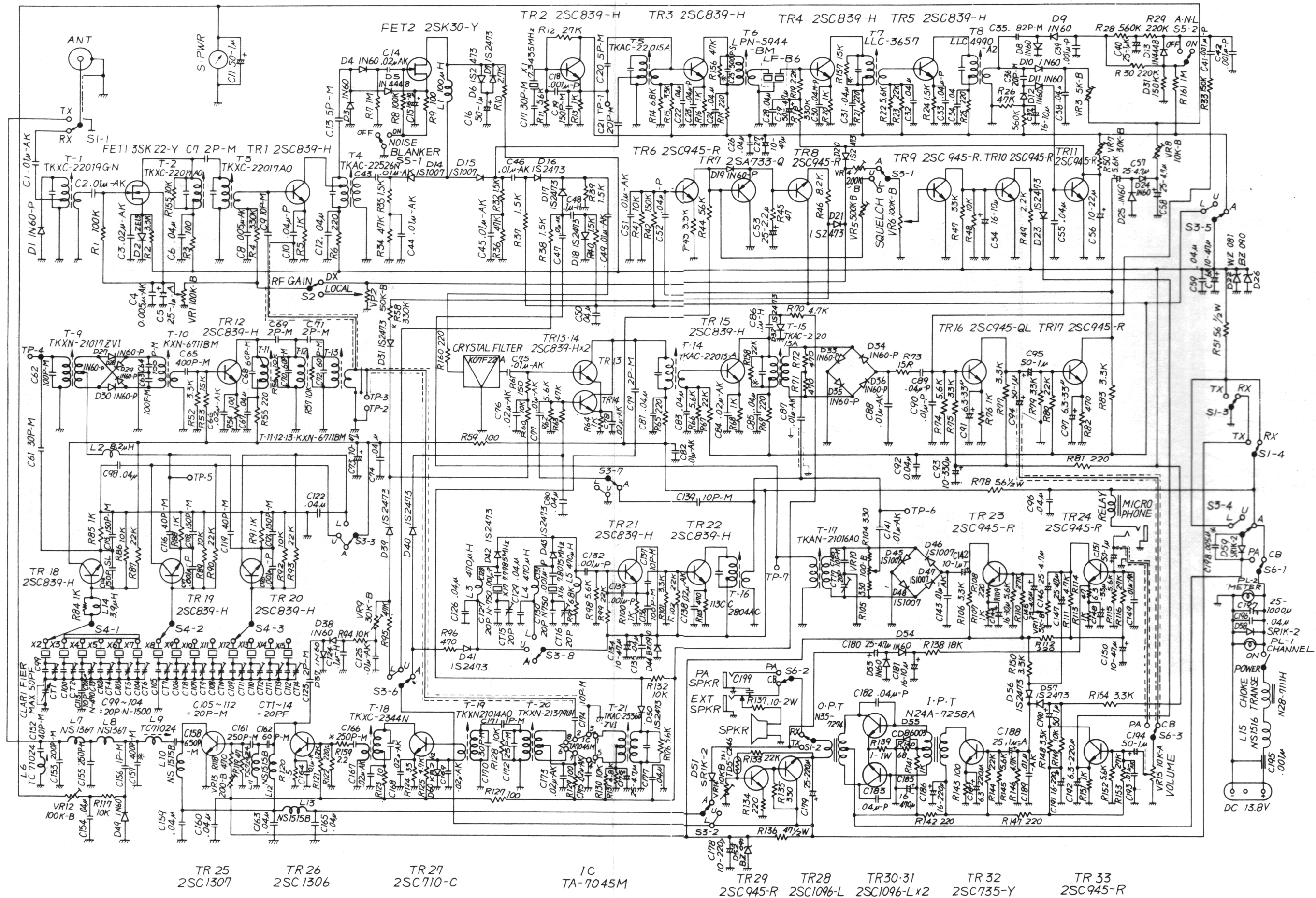
FIGURE 8, SCHEMATIC DIAGRAM
