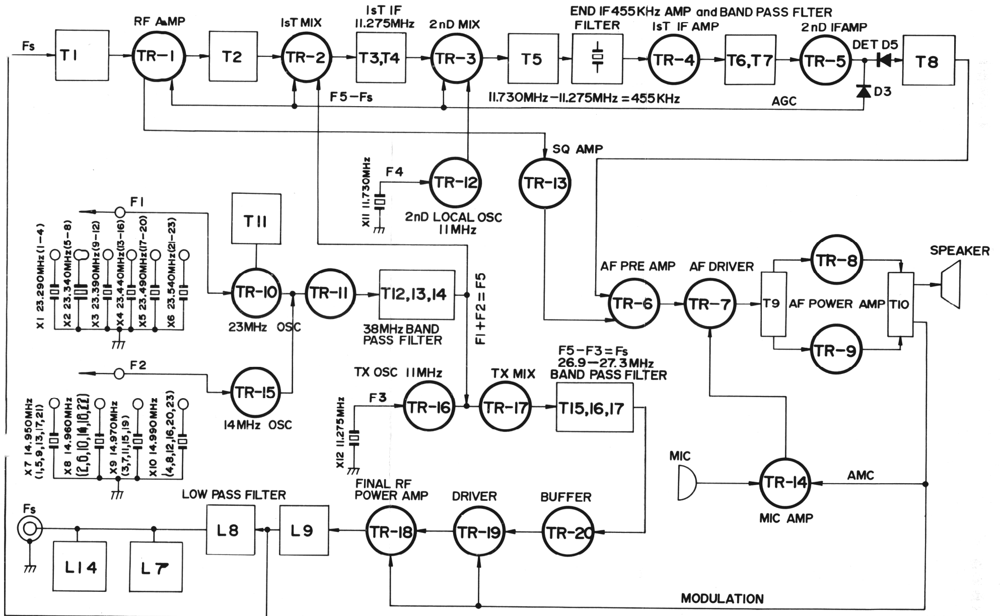
FIGURE 2, BLOCK DIAGRAM
