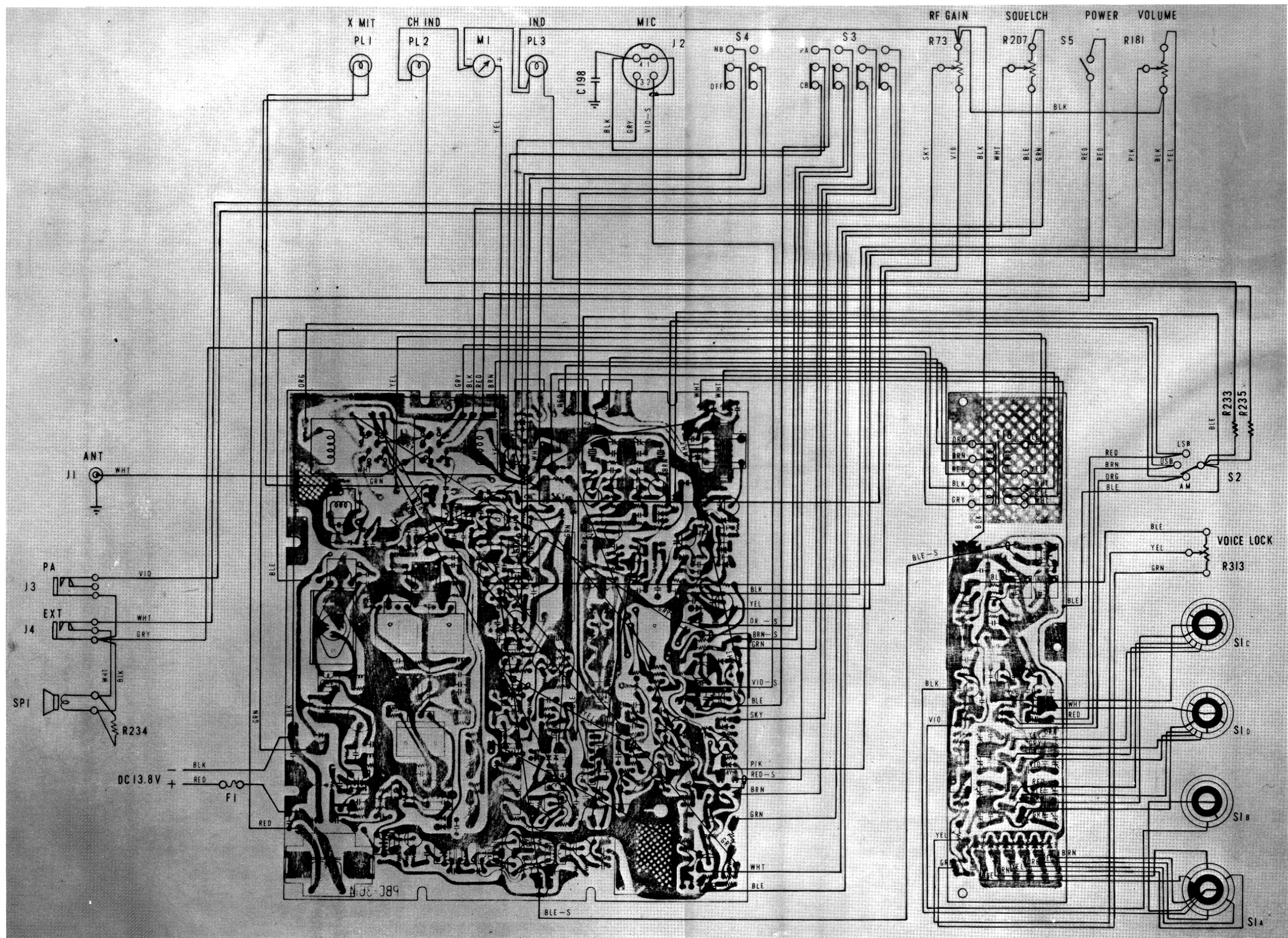
WIRING DIAGRAM COBRA 132(A) Fig 19
