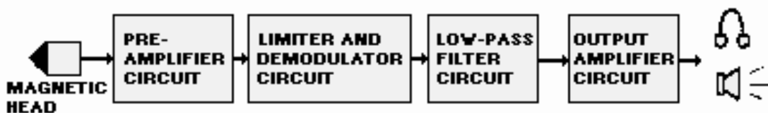
Figure 5-5.—FM reproduce electronics.
