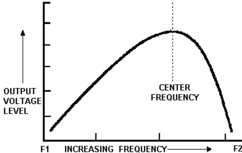
Figure 6-2.—Frequency response of a reproduce head.
