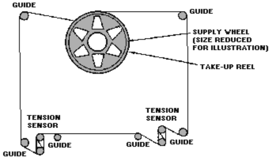
Figure 4-8.—Co-axial tape reeling configuration.
