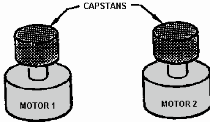
Figure 4-12.—Dual-motors dual capstans drive system.
