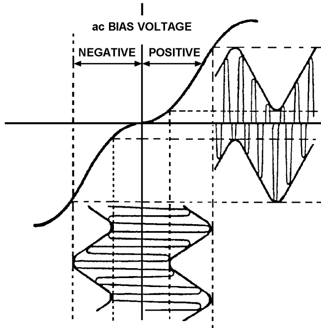
Figure 1-3.—Magnetic recording with ac bias voltage.
