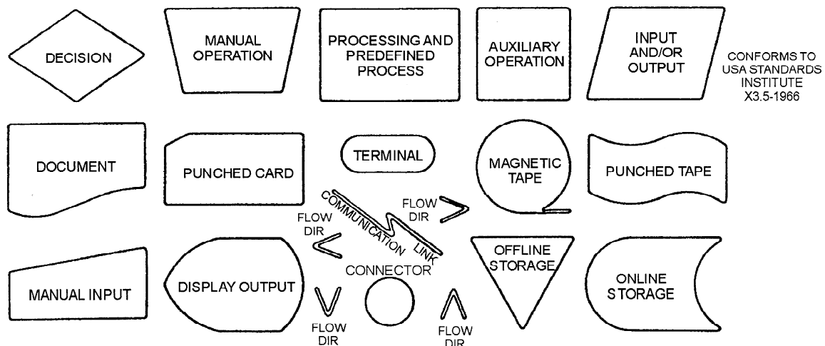
Figure 3-4.—Flowchart template.
