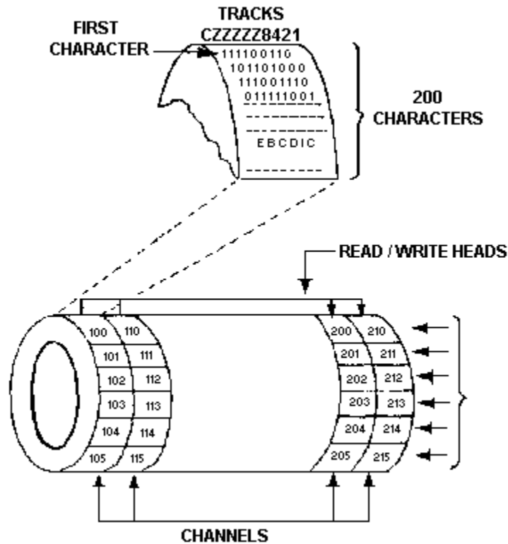
Figure 2-16.—Magnetic drum.
