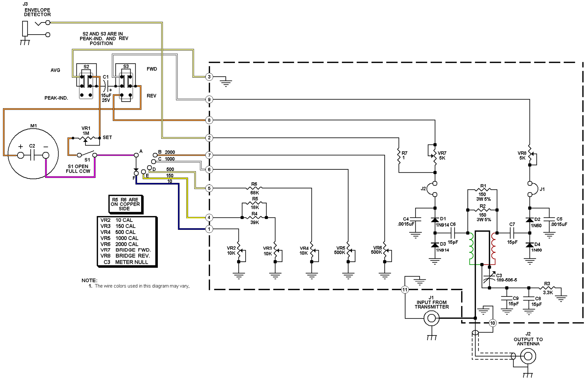
Outcom Wattmeter PW-2000 Copyright © 2006, CBTricks.com All Rights Reserved CBTricks.com Rev.#1.1
