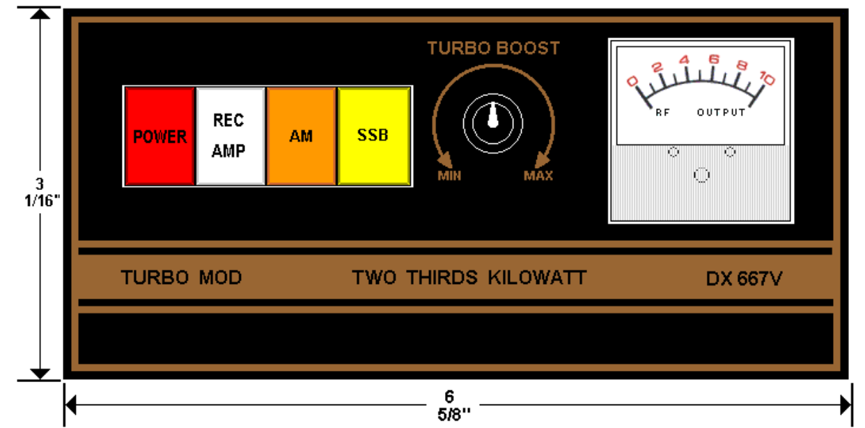
DX 667V Turbo Mod Front View
