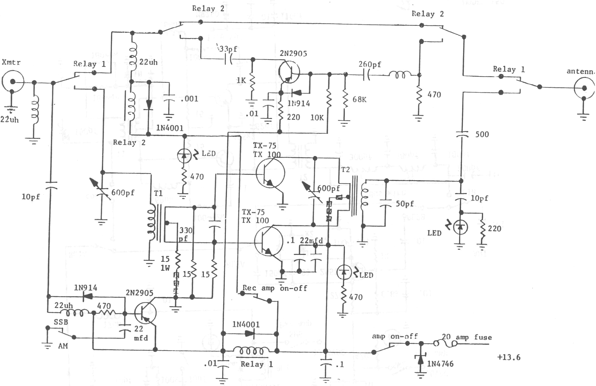
MODEL TX-100 AND TX-75 LINEAR AMPLIFIER PALOMAR ELECTRONICS CORP. ESCONDIDO, CALIFORNIA
